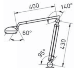
Task Light KL 36 36 W, Clour: light grey mounting clamp for ergo S+P
